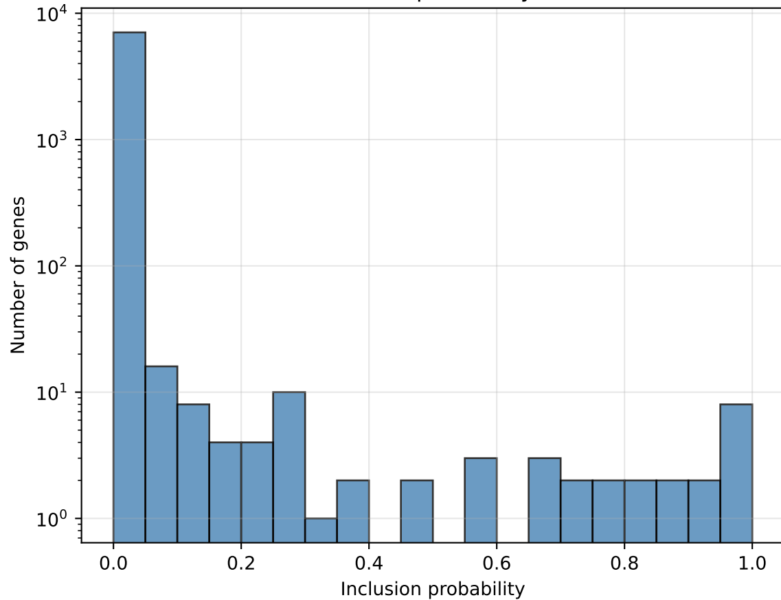
SVM-RFE: inclusion probability distribution
