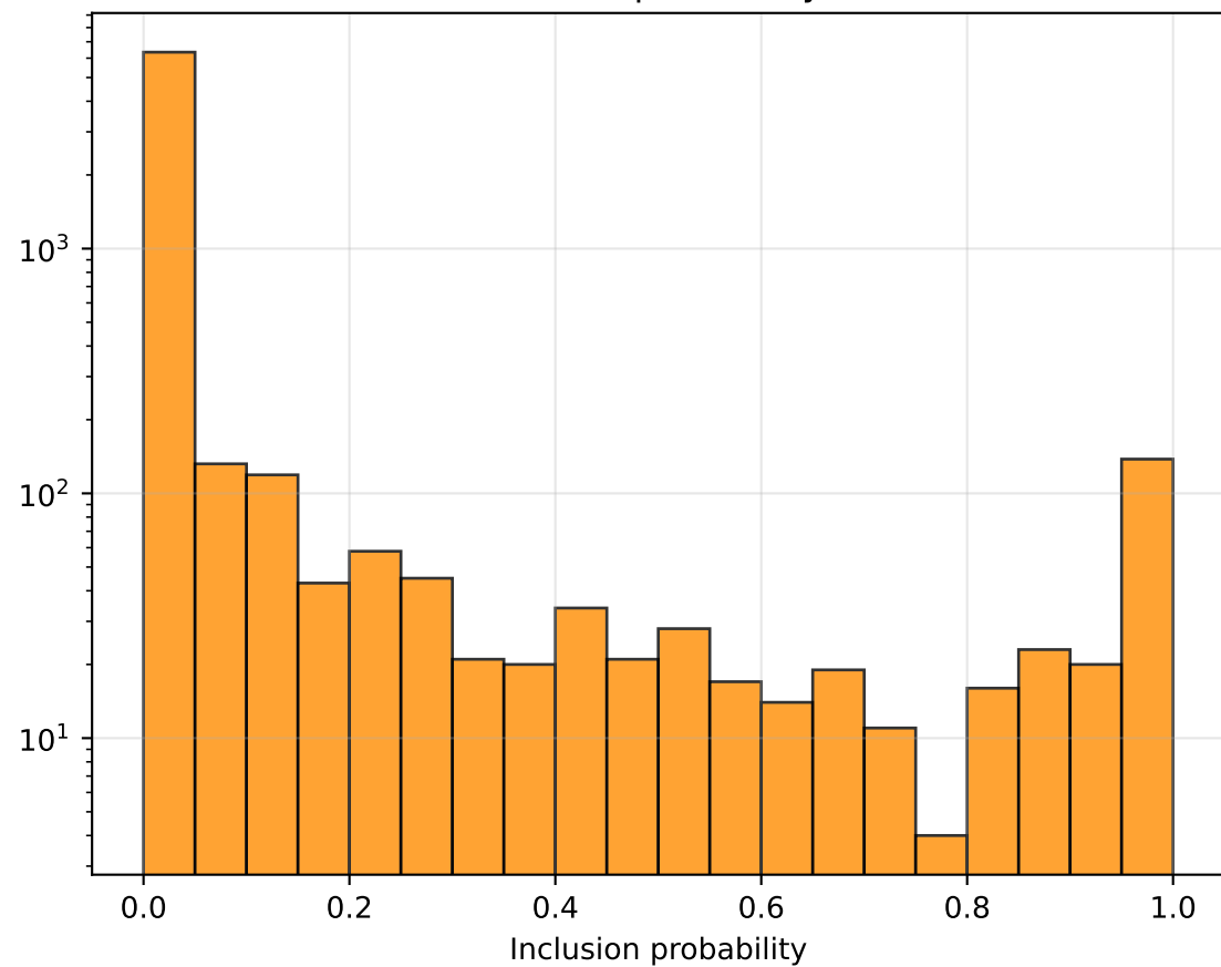
FDR (BH): inclusion probability distribution
