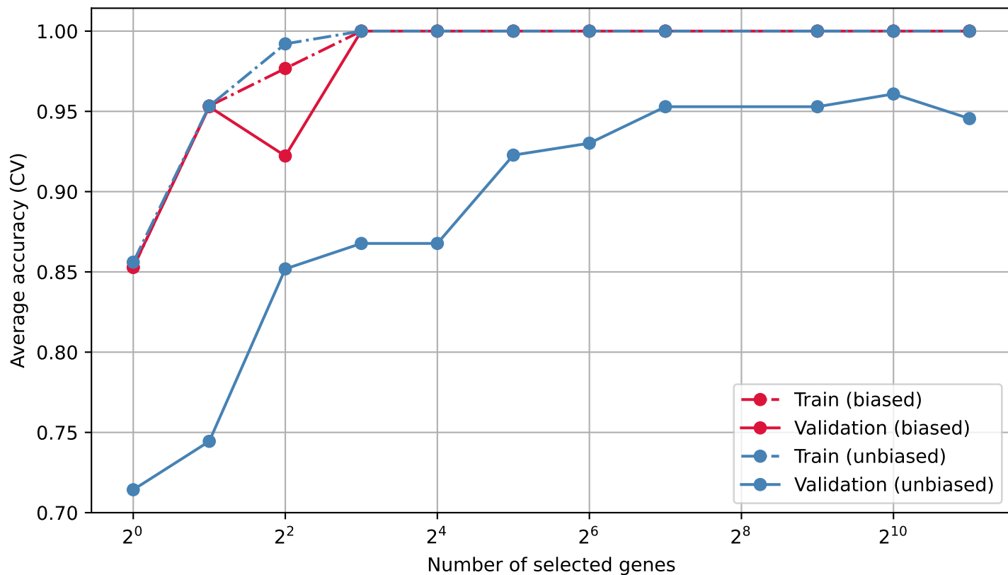
RFE
