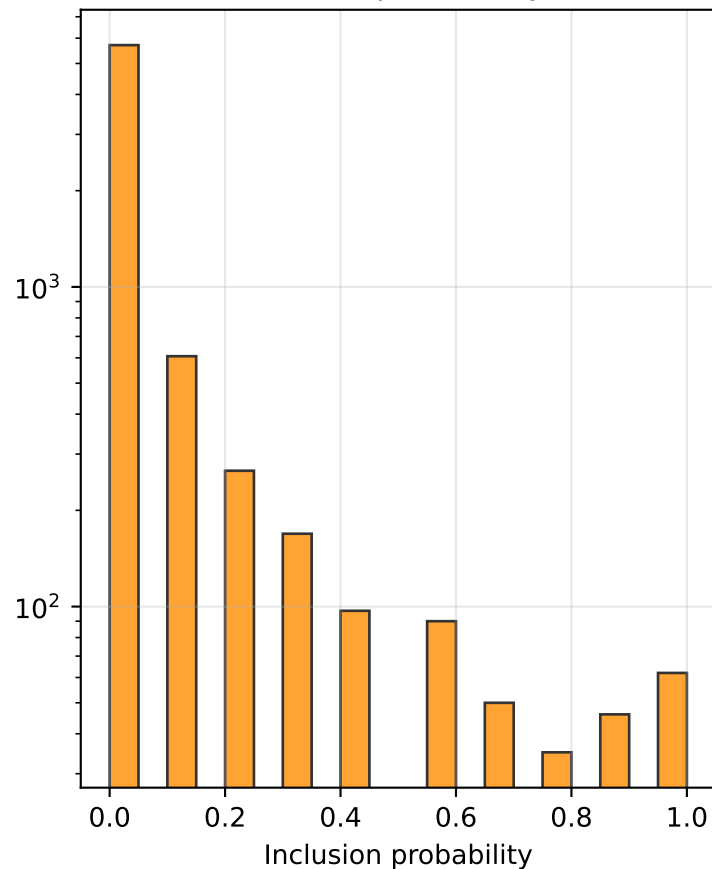
FDR (BH): inclusion probability distribution
