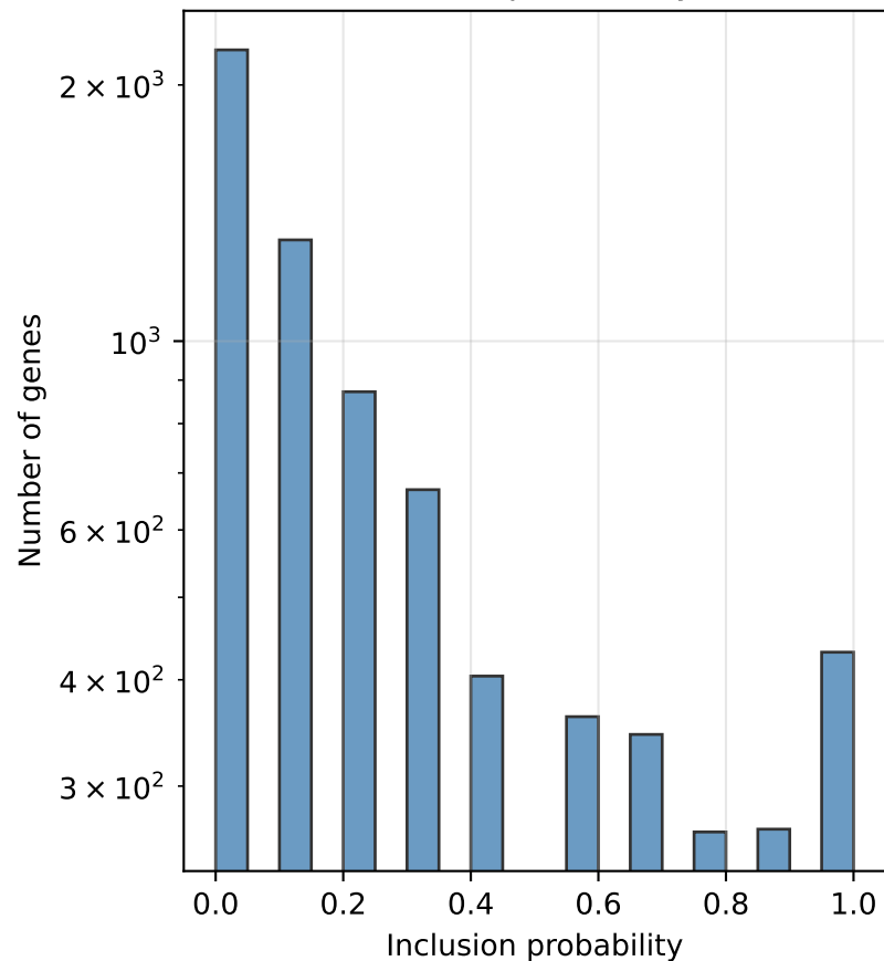
SVM-RFE: inclusion probability distribution
