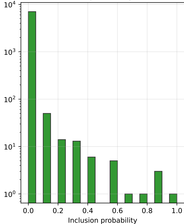
Lasso: inclusion probability distribution
