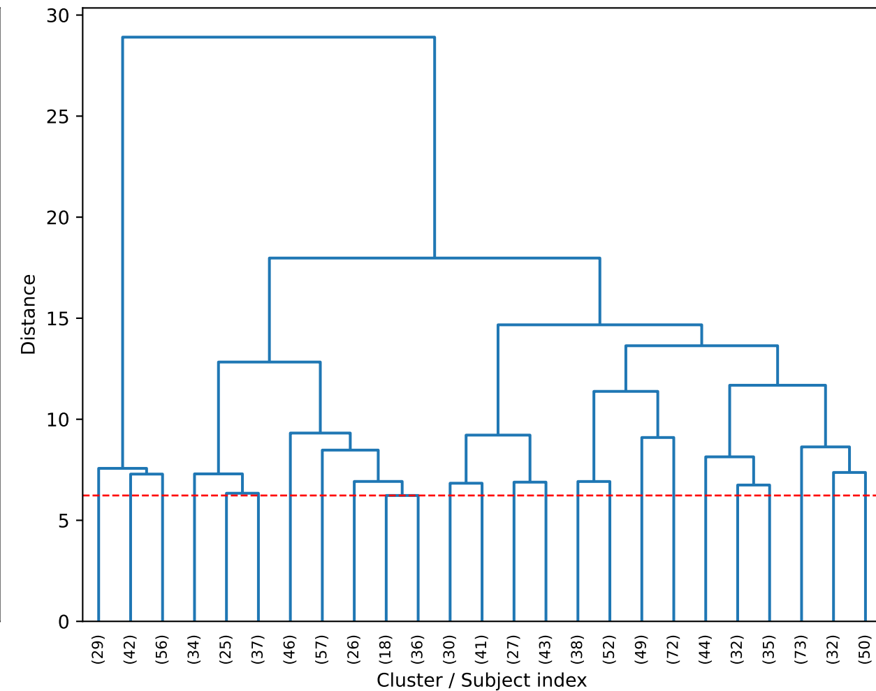
Class 2 → 25 clusters
