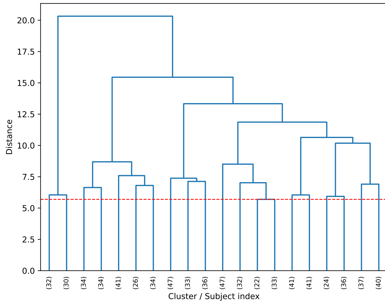
Class 0 → 20 clusters
