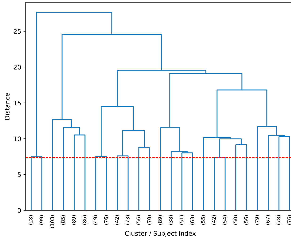
Class 1 → 25 clusters
