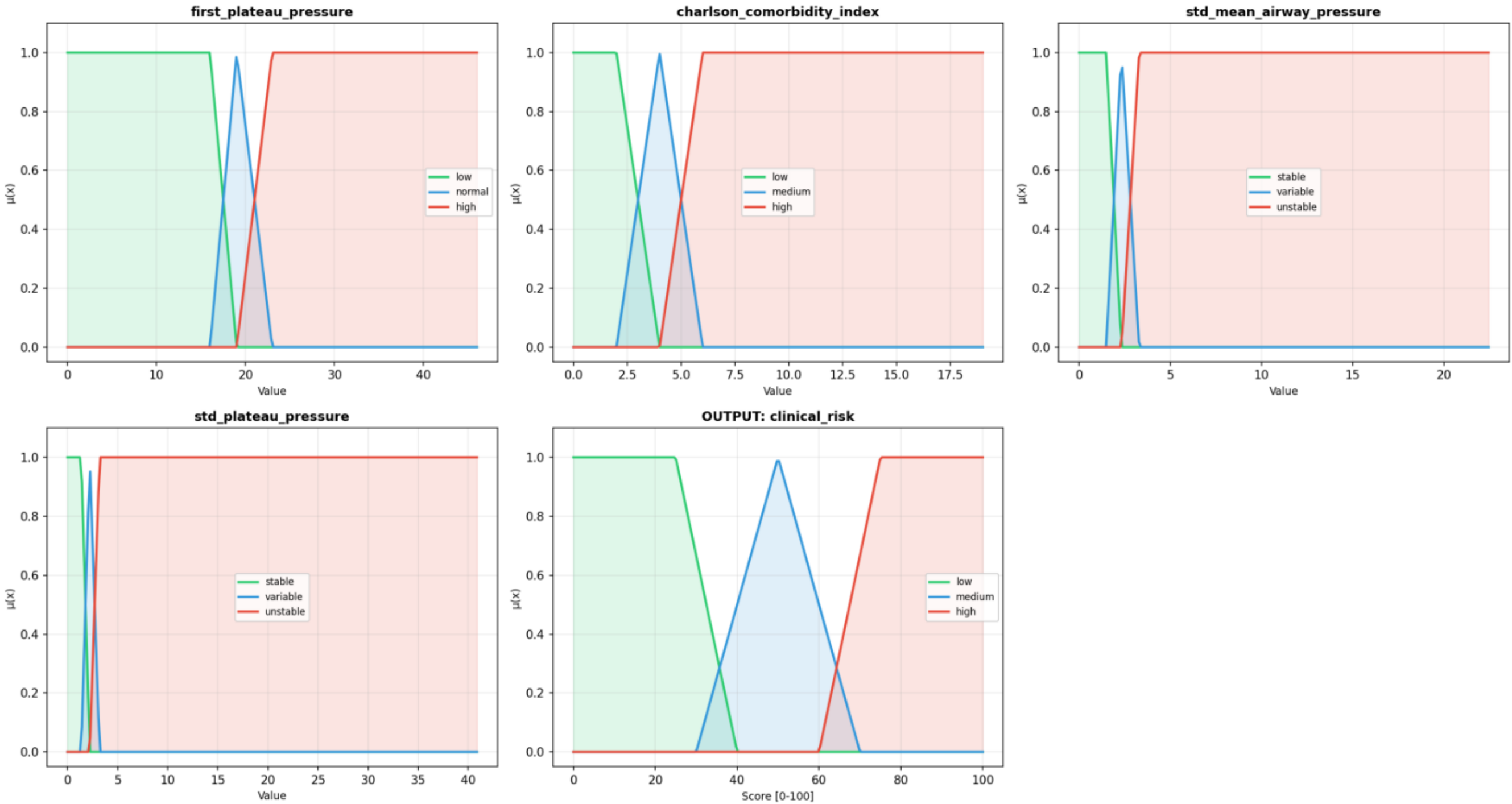
LAB4 - Cluster 4: Membership Functions (Feature Continue + Output)
