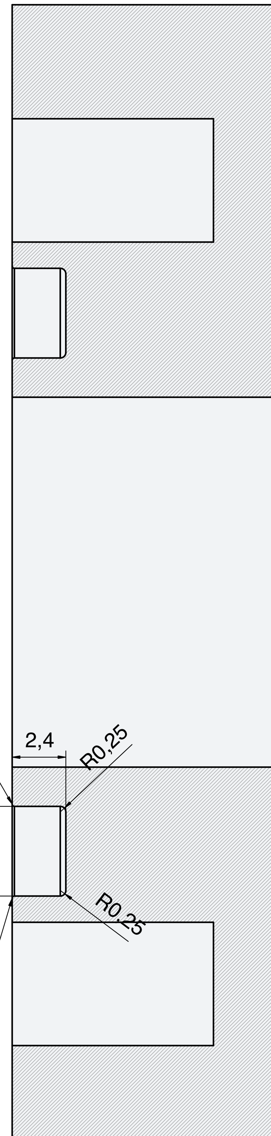
Section B-B
