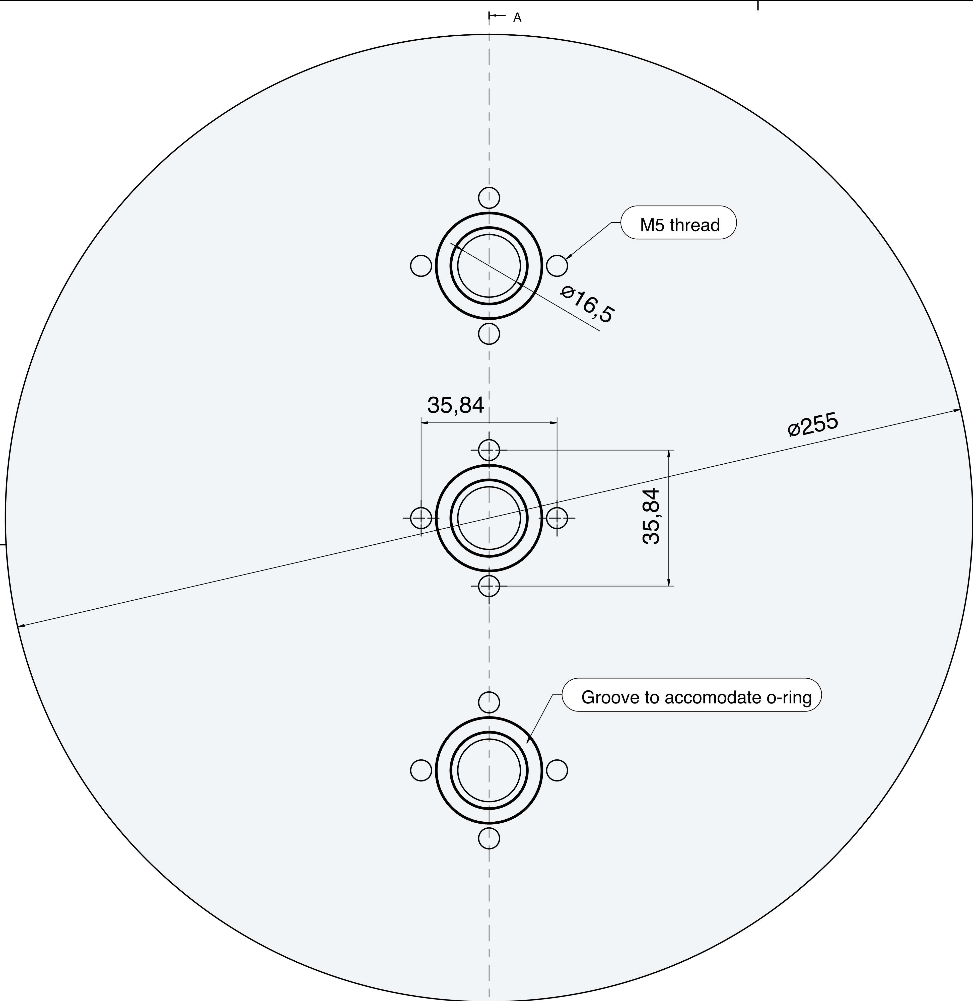
Top view
