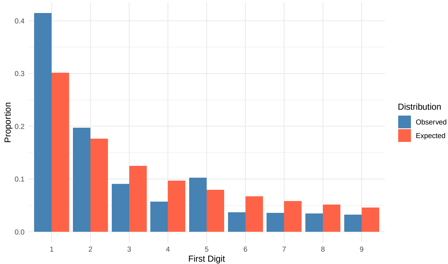
First-Digit Distribution vs Benford's Law
