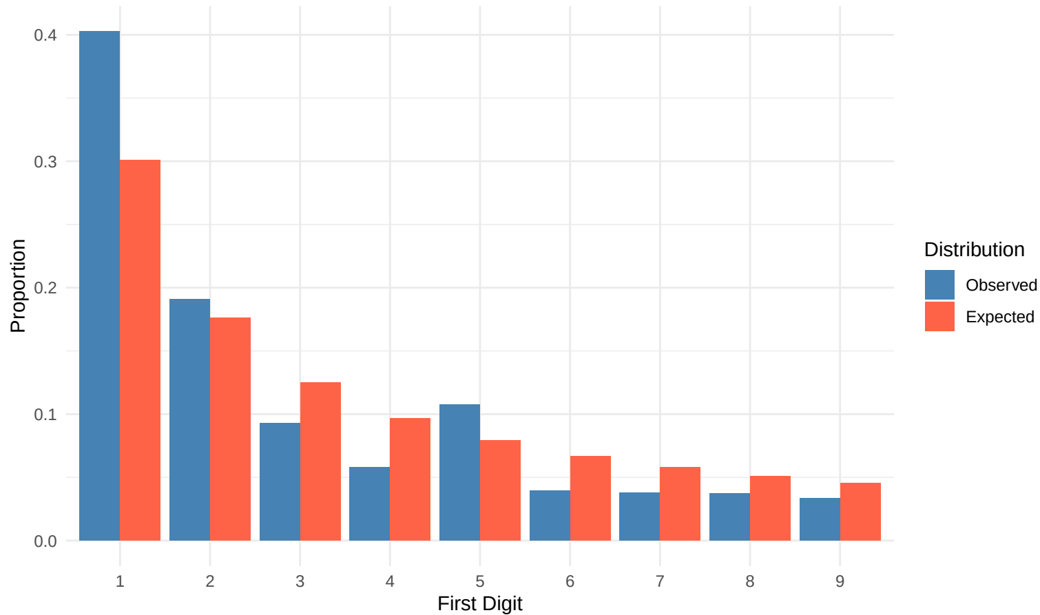
First-Digit Distribution vs Benford's Law
