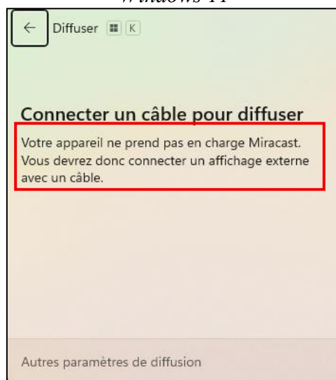
Windows 11
