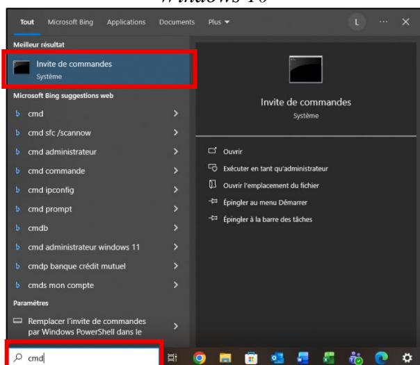
Windows 10
