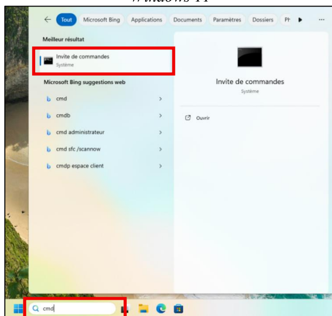
Windows 11
