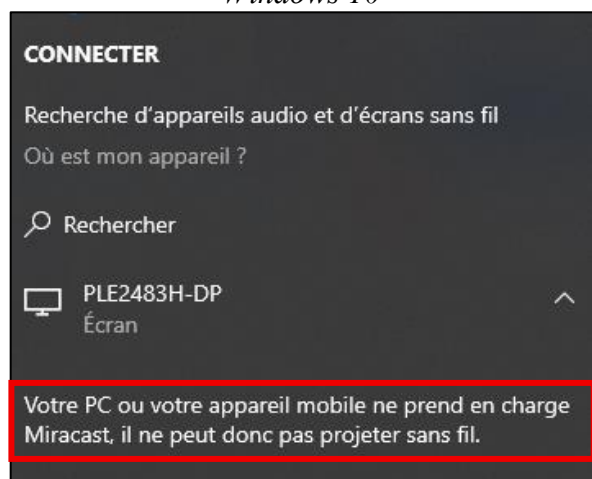
Windows 10
