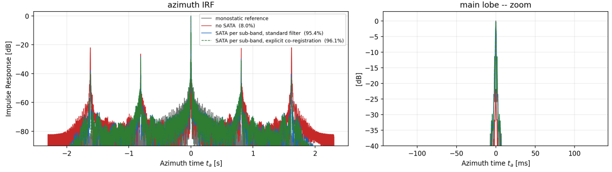
Figure 3: The full pipeline. The dashed green (explicit co-registration) tracks the solid blue (standard) everywhere, including the residual ambiguities at \pm 0.87 s.
