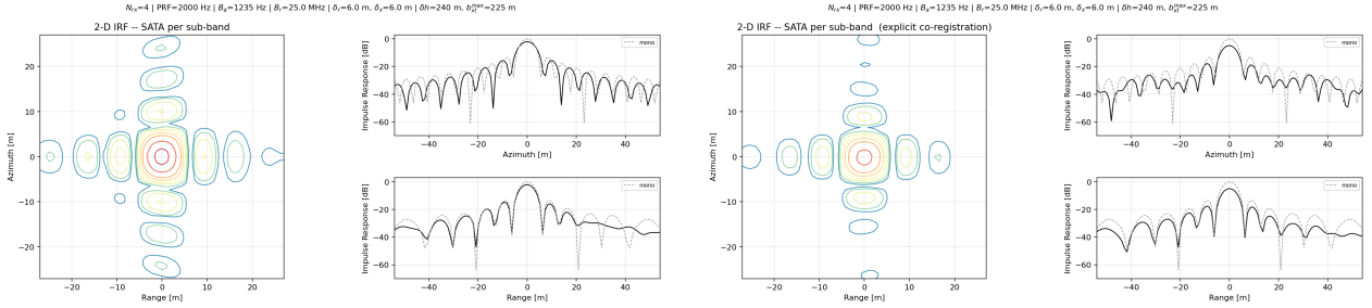
Figure 4: 2-D impulse response, standard pipeline (left) against the explicit co-registration (right), both with SATA per sub-band, at \delta_r = \delta_x = 6 m. Azimuth/range PSLR -13.64/-12.55 dB and -13.04/-12.66 dB respectively; IRW 5.56/4.18 m and 4.63/4.18 m. Produced by run_irf2d.py , with and without -coreg .
