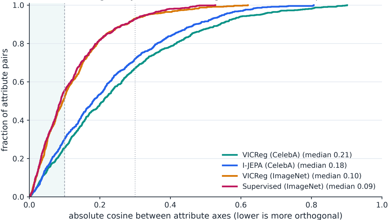
Orthogonality across all 735 eligible CelebA attribute pairs
