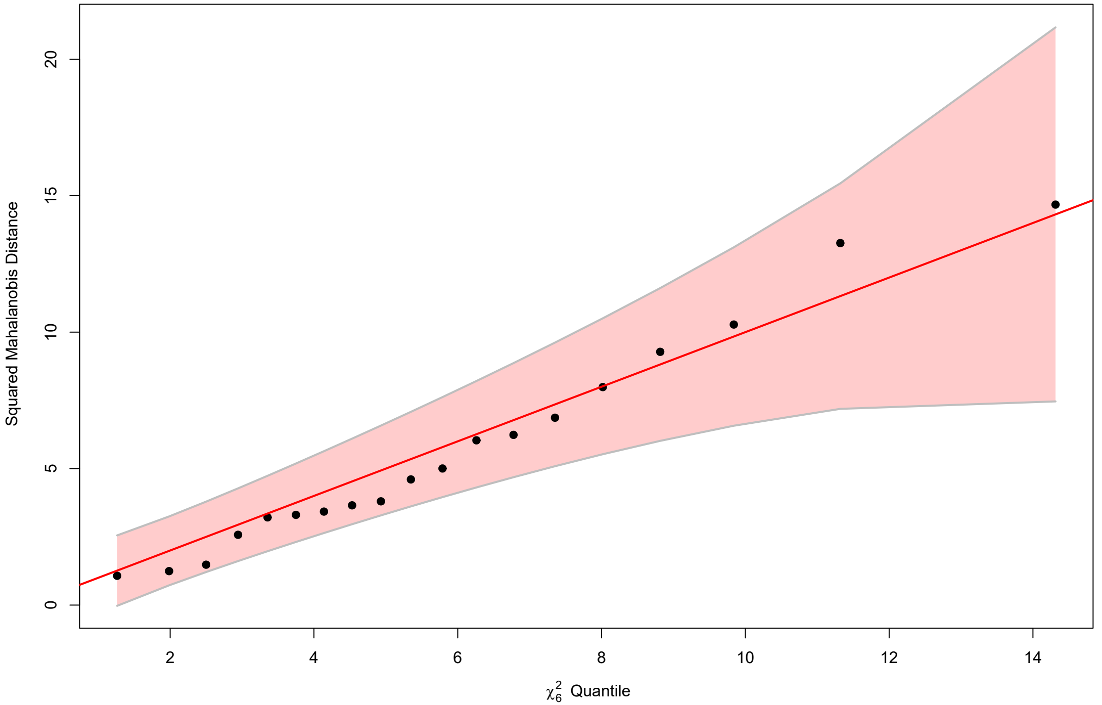
Chi-Square Q-Q Plot of Carros
