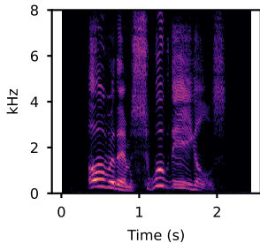
Clean STFT
