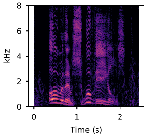
Adversarial STFT
