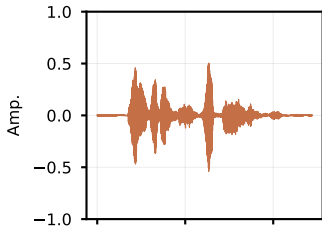
Adversarial STFT
