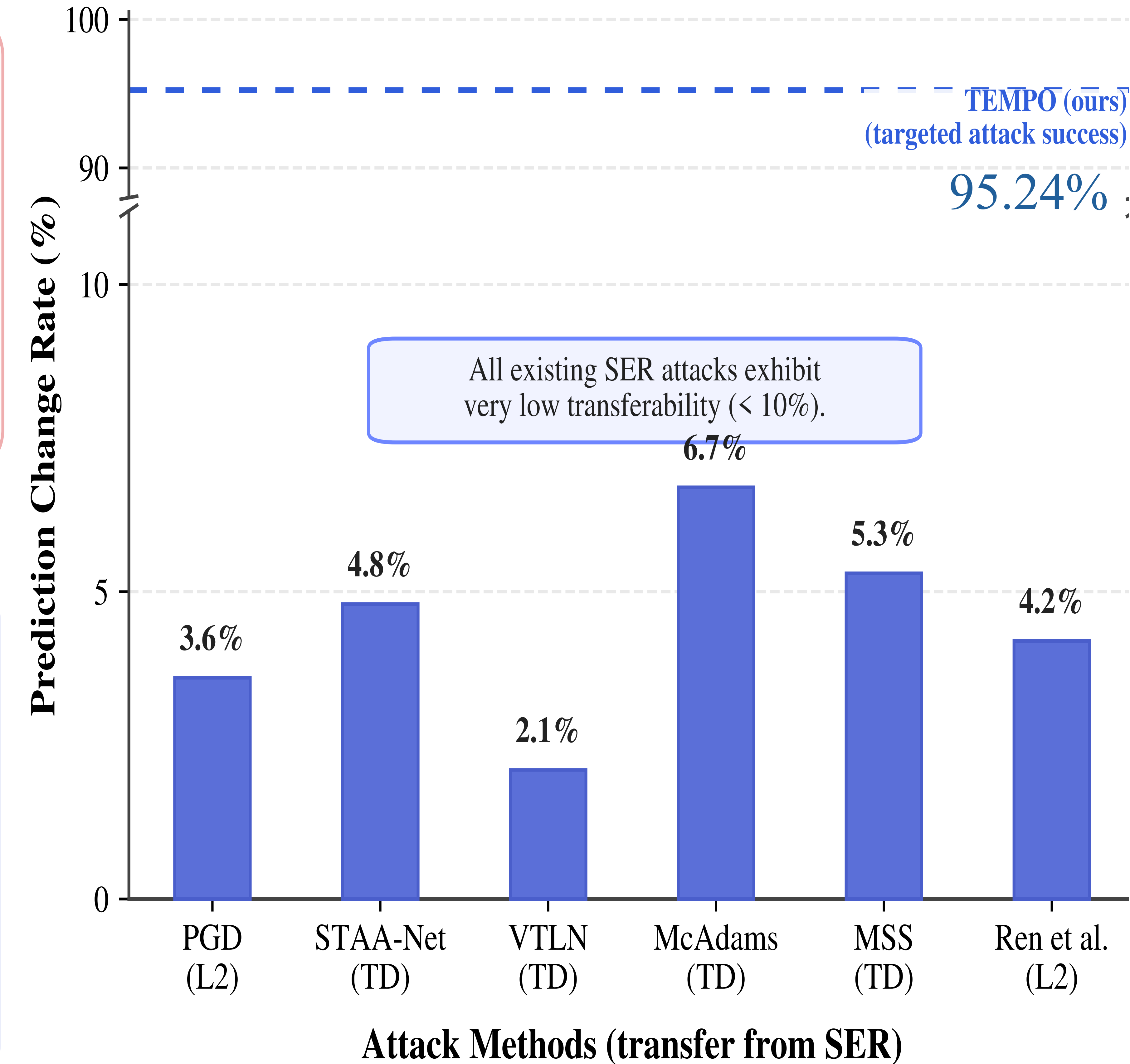
(B) Transfer Attack Failure on Audio LLMs
