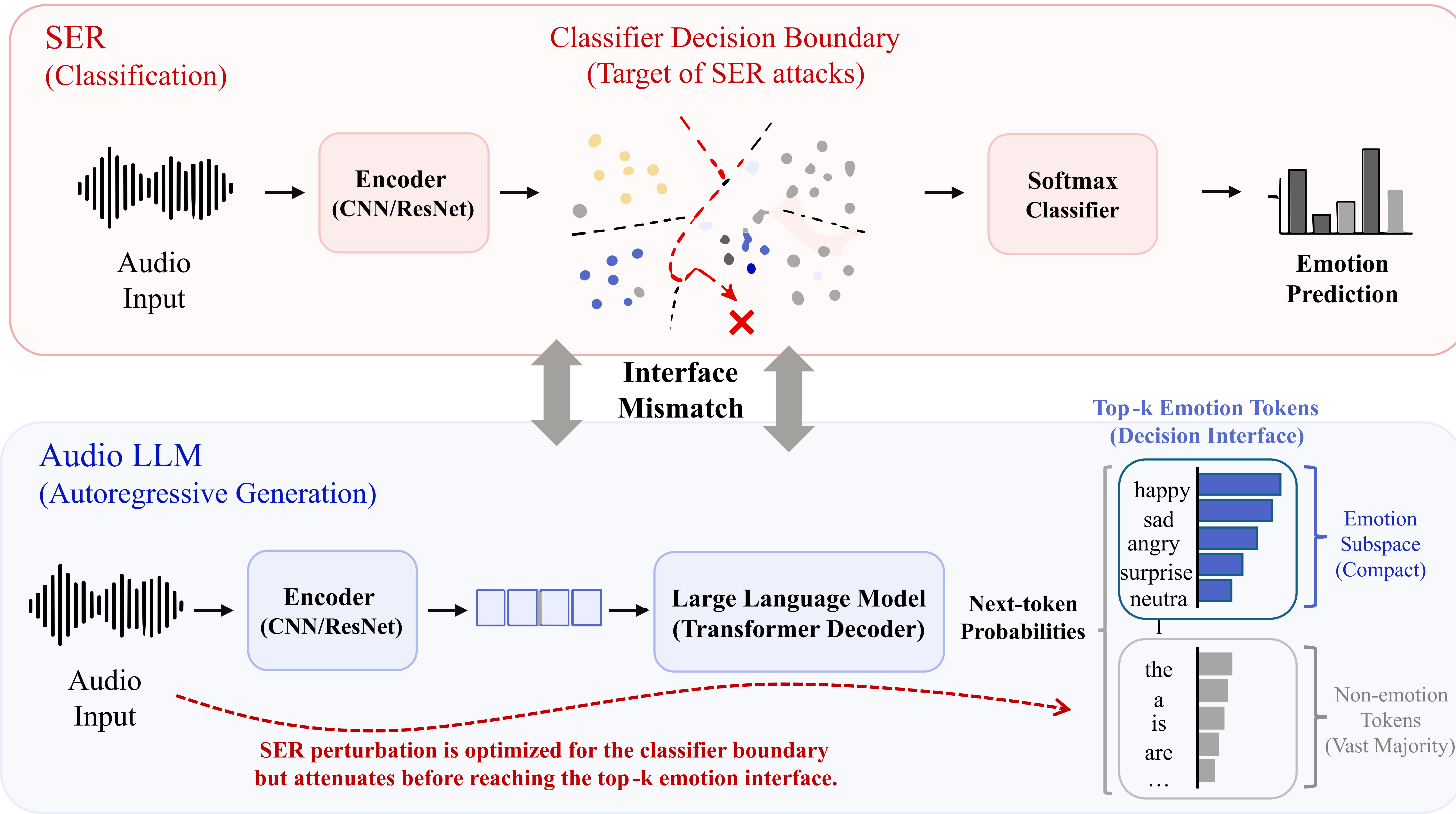
(A) Decision Interface Mismatch: SER vs Audio LLM
