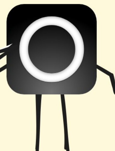
Kosuke
