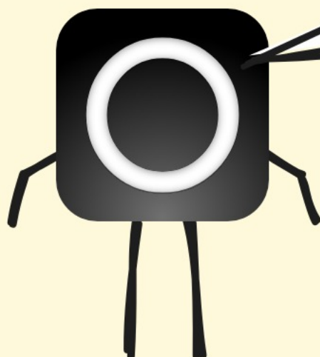
Kosuke
