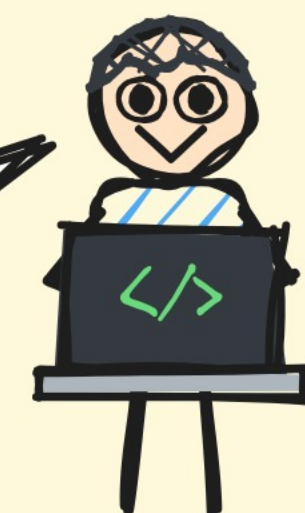
dev
