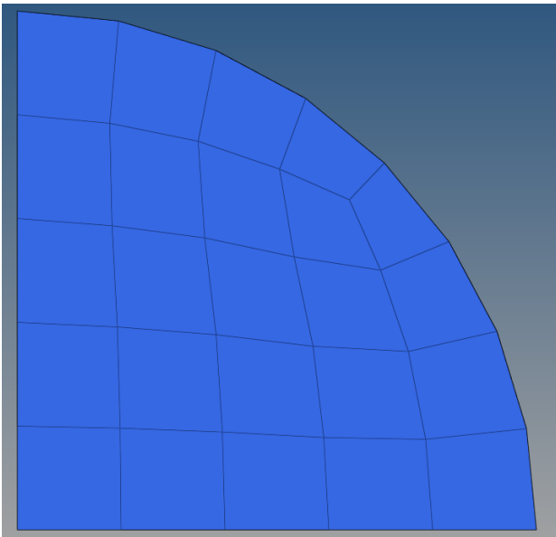
FIGURE 2 – Maillage surfacique (Quad only)
