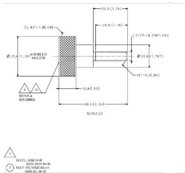
FIGURE 28 – P07 de l'outillage 956A8403G02
