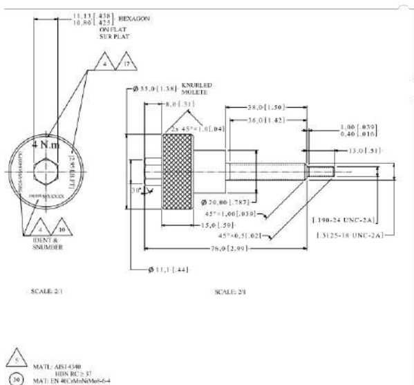
FIGURE 29 – P30 de l'outillage 956A8403G03
