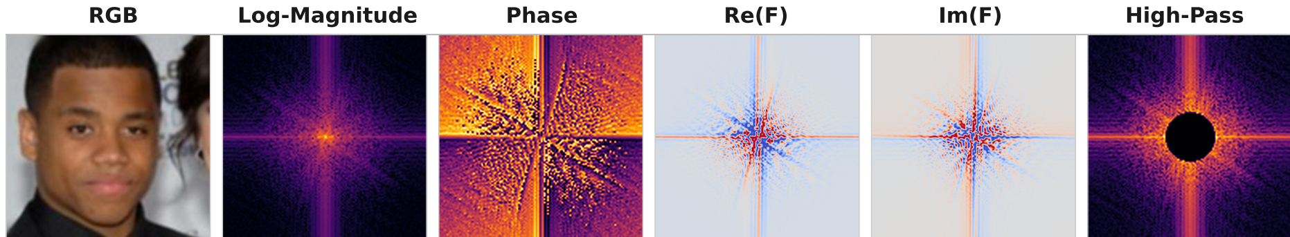
Class 0 (Real)
