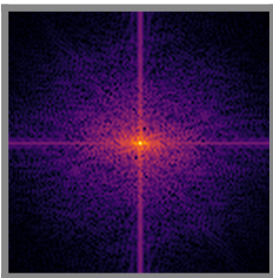
\log(|\mathcal{F}| + 1)
