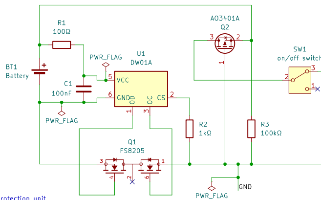
Battery protection unit
