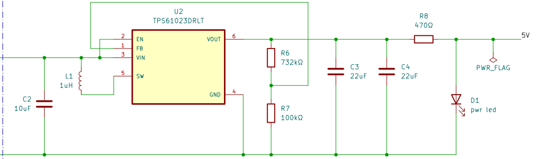
5V boost converter unit
