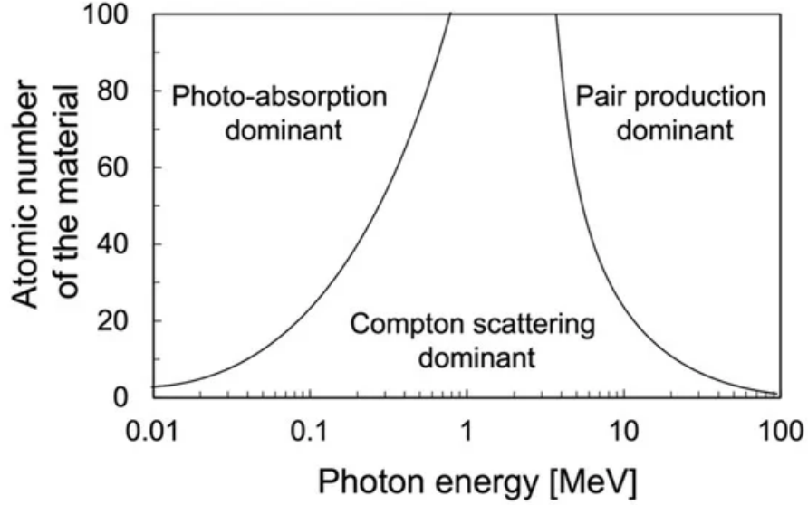
Figure 3: Relative importance of photoelectric effect, Compton scattering and electron-positron pair creation as a function of the energy of the incoming photon and the atomic number Z of the scatterer material.
