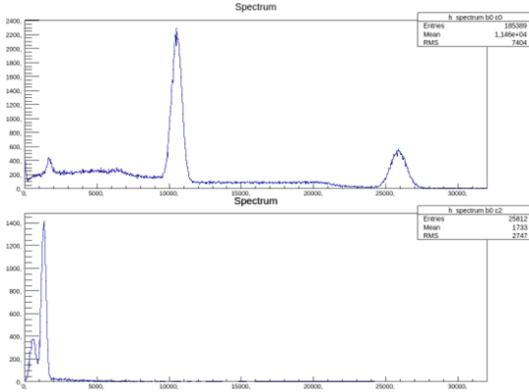
Figure 7: Typical energy spectra with the source of Sodium (top) and Americium (bottom).
