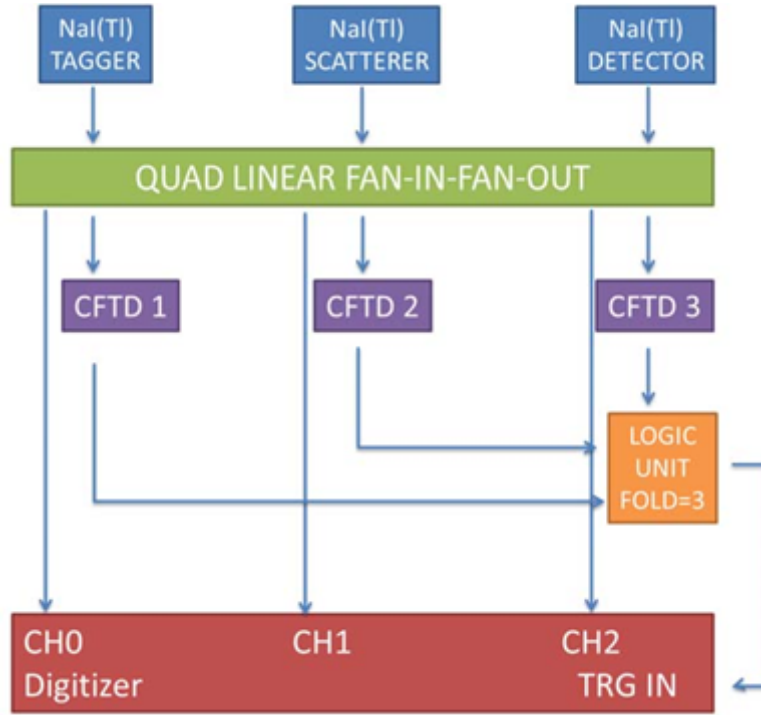
Figure 5: Electronics Diagram for the Compton Experiment.
