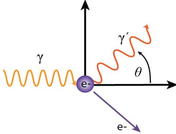
Figure 1: Schematic representation of the Compton scattering
