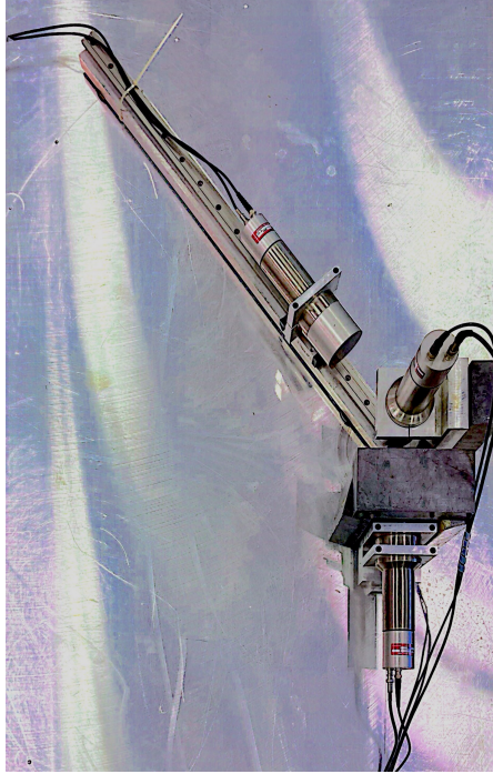
Figure 4: Experimental setup for the study of Compton scattering.
