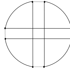
c) Non-sequential 4-Opt move
