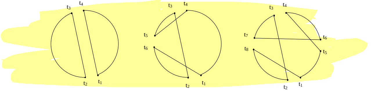
Figure 5. Lin-Kernighan's infeasibility moves.
