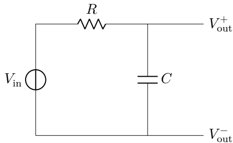
Figure 1: Passive RC low-pass filter with cutoff f_c = 1/(2\pi RC) .
