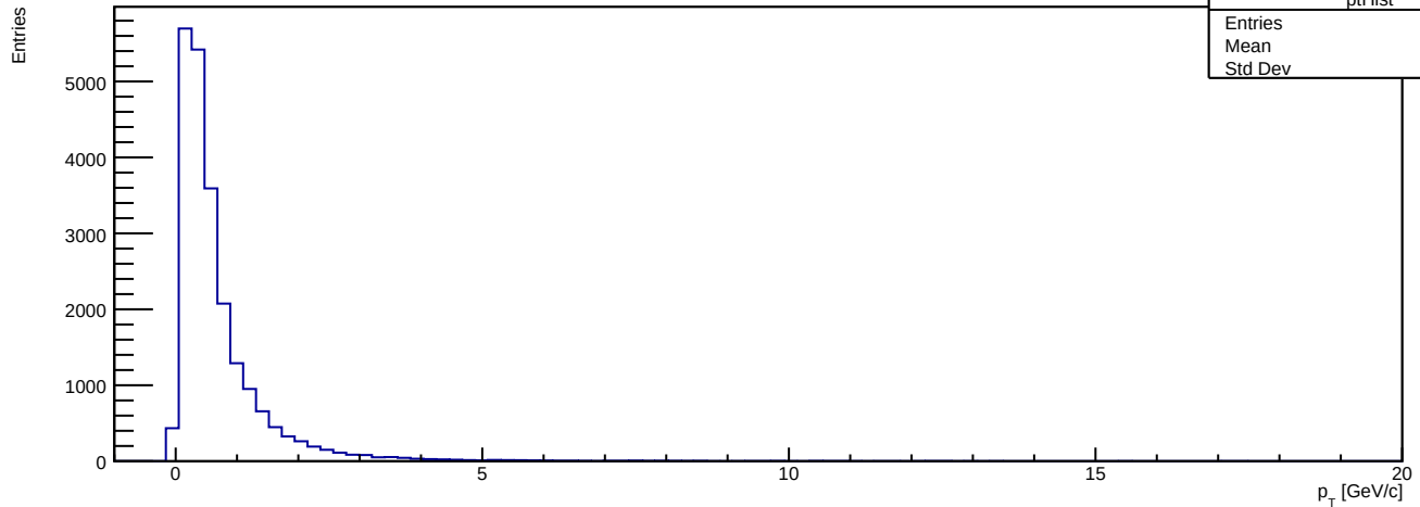
Charged Particle p_T
