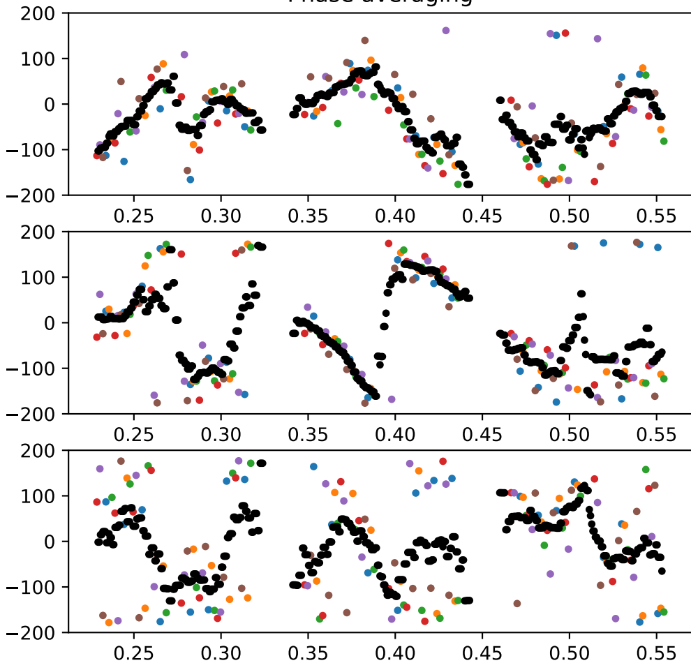
Phase averaging
