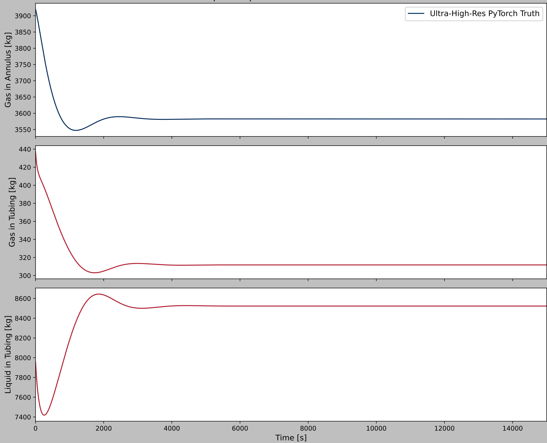
Open-Loop Simulation of Gas-Lift Well
