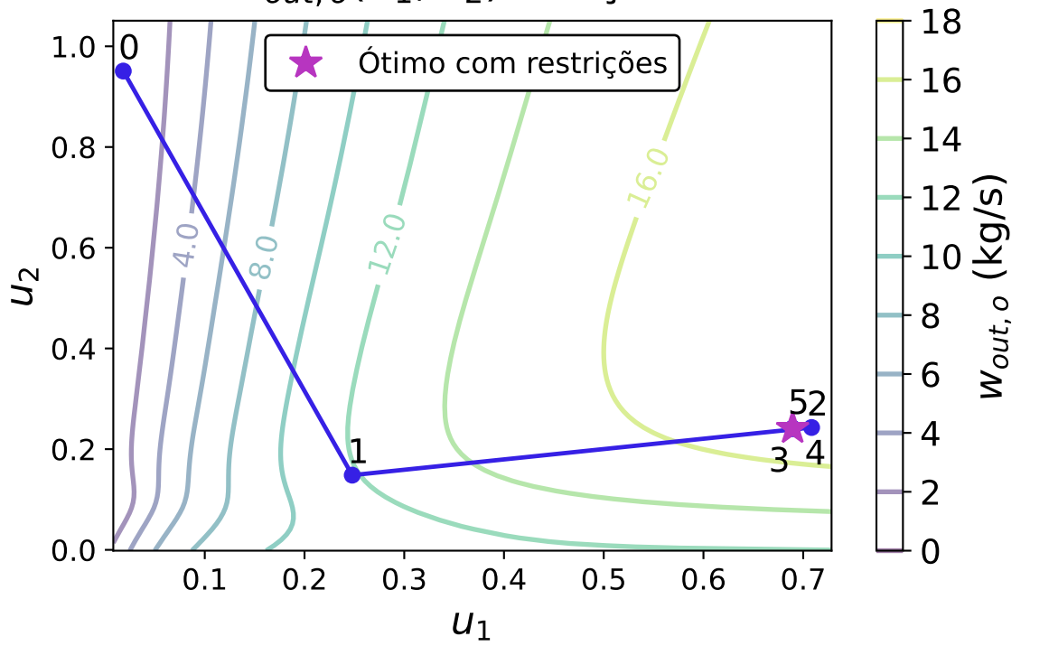
w_{out,o}(u_1, u_2) - Poço P2
