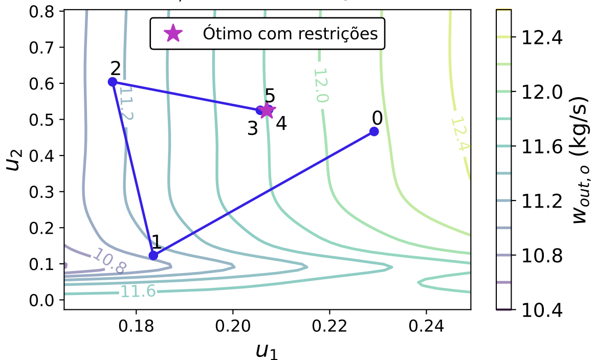
w_{out,o}(u_1, u_2) - Poço P1
