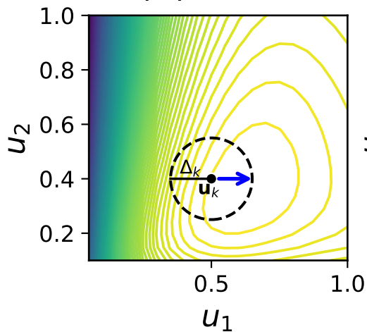
\tilde{r}(\mathbf{u}) - PINN
