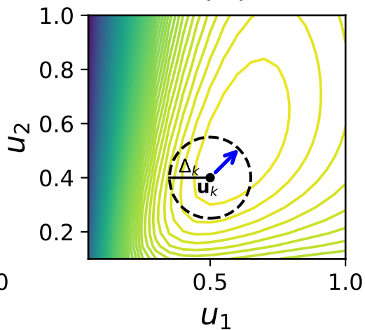
s(\mathbf{u})
