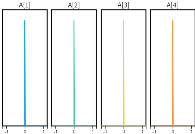
Histogramas de A^{[1]}, \dots, A^{[4]} com \theta = 0 .
