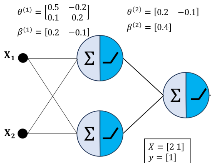
Figure 1: Multilayer Perceptron
