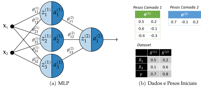
Figure 1: Perceptron Multicamadas
