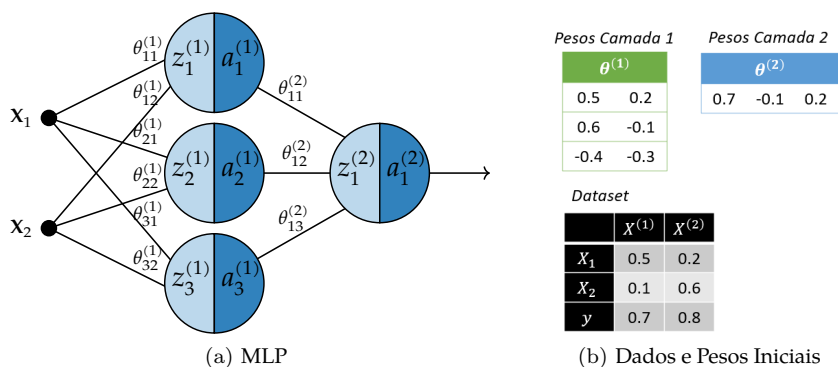
Figure 1: Perceptron Multicamadas
