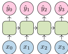
many-to-many
