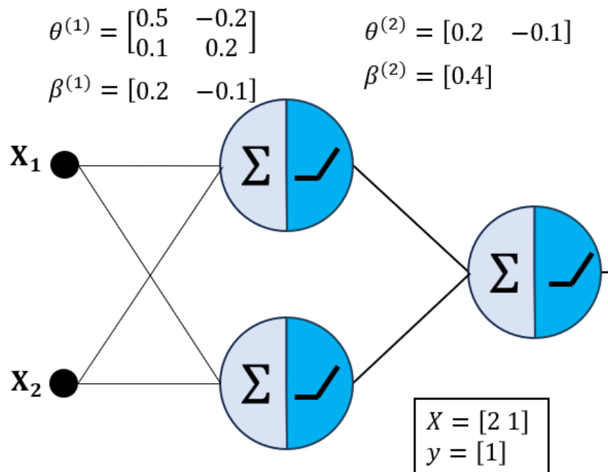
Figura 1: Multilayer Perceptron
