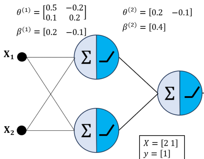
Figure 1: Multilayer Perceptron
