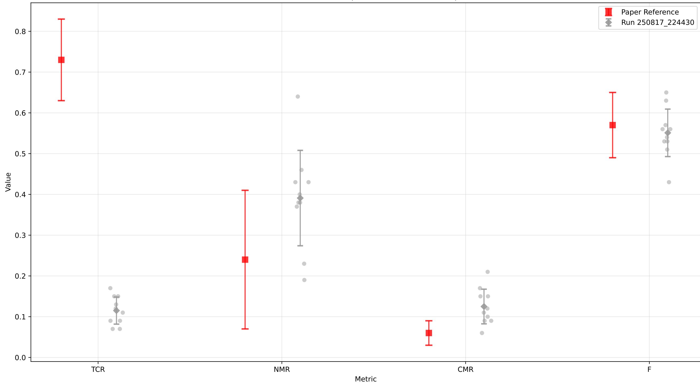
Model Performance Metrics: Paper Reference vs Our Implementation
