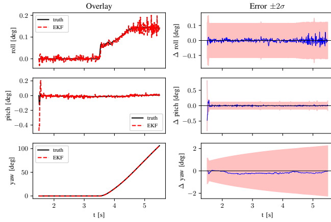
Fig. 2. Orientation data and 2\sigma errors for first test case. Maximum error in yaw is \approx 1^\circ , while the other angles had error bounds on the order of 0.1^\circ respectively.
