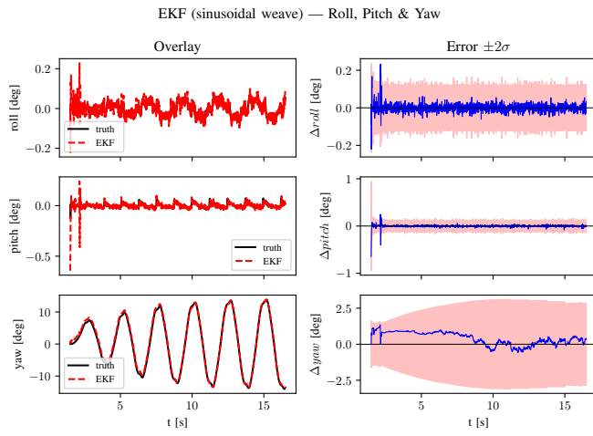
Fig. 4. Orientation data and 2\sigma errors for second test case. Maximum error in yaw is \approx 1^\circ , while the other angles had error bounds on the order of 0.1^\circ respectively..
