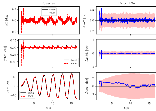
Fig. 4. Orientation data and 2\sigma errors for second test case. Maximum error in yaw is \approx 1^\circ , while the other angles had error bounds on the order of 0.1^\circ respectively..
