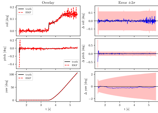
Fig. 2. Orientation data and 2\sigma errors for first test case. Maximum error in yaw is \approx 1^\circ , while the other angles had error bounds on the order of 0.1^\circ respectively.
