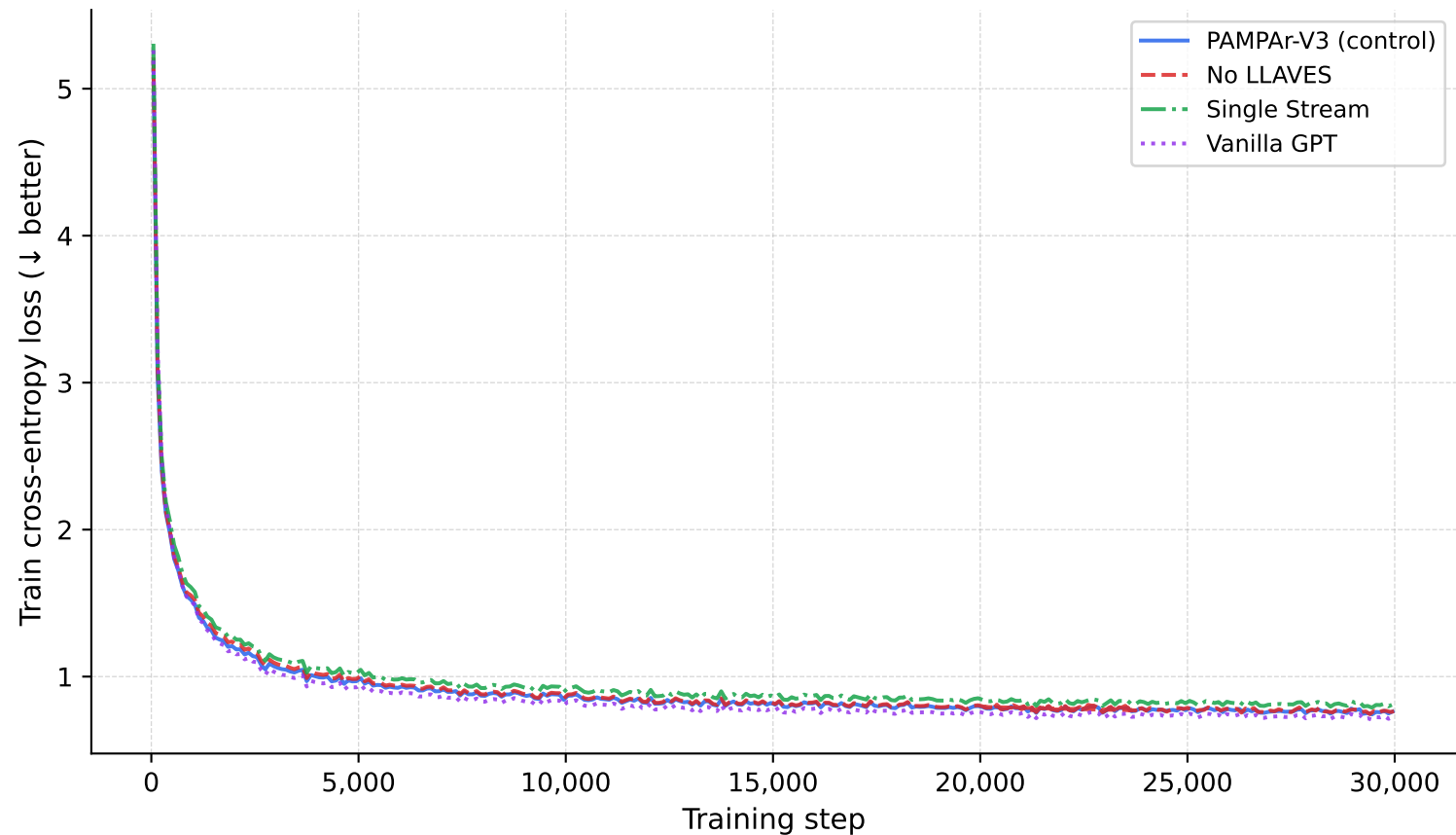
PAMPAr Ablation — Train Loss (100-step avg) vs. Training Step
