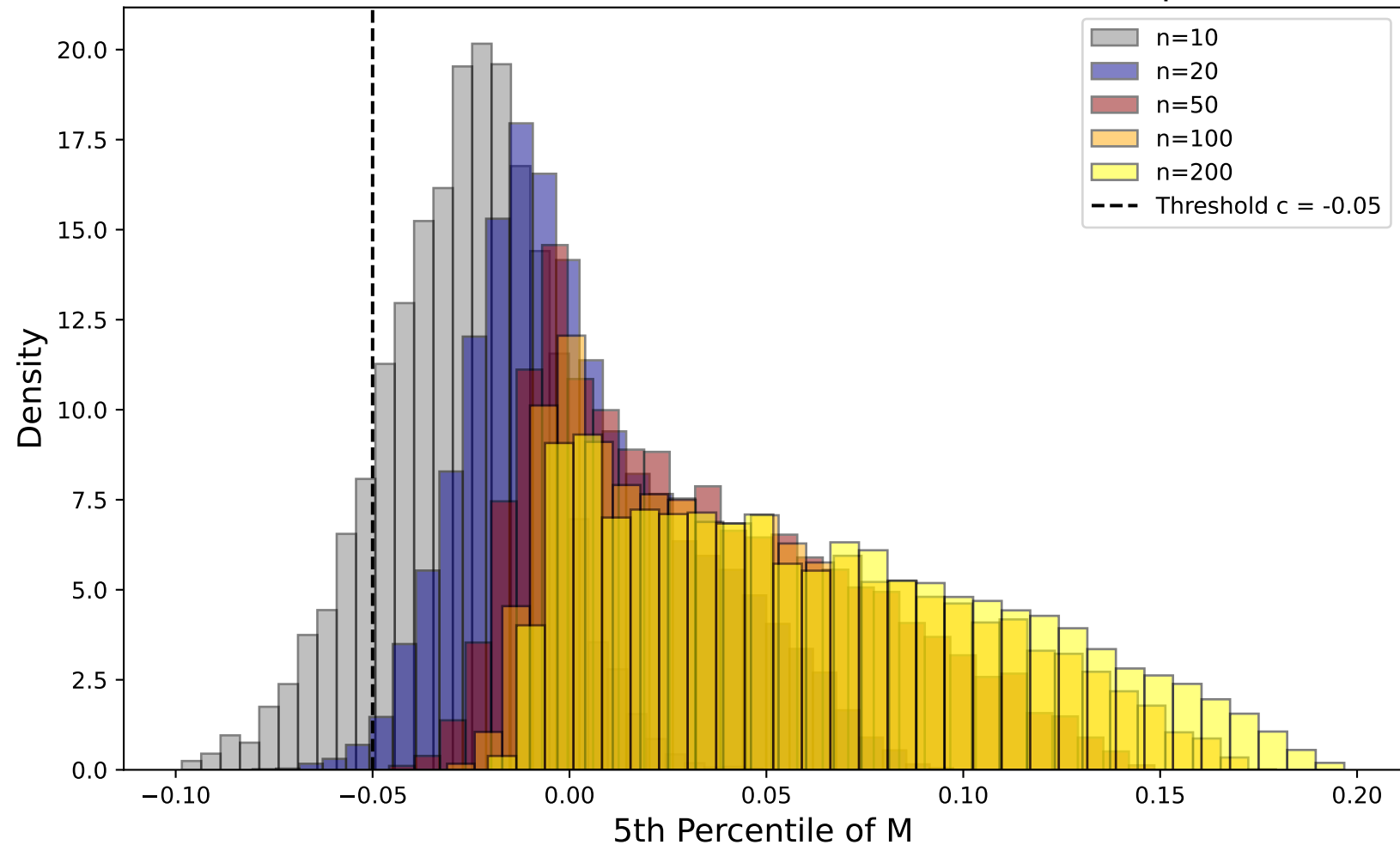
Shift in Distribution of 5th Percentile of M with Sample Size
