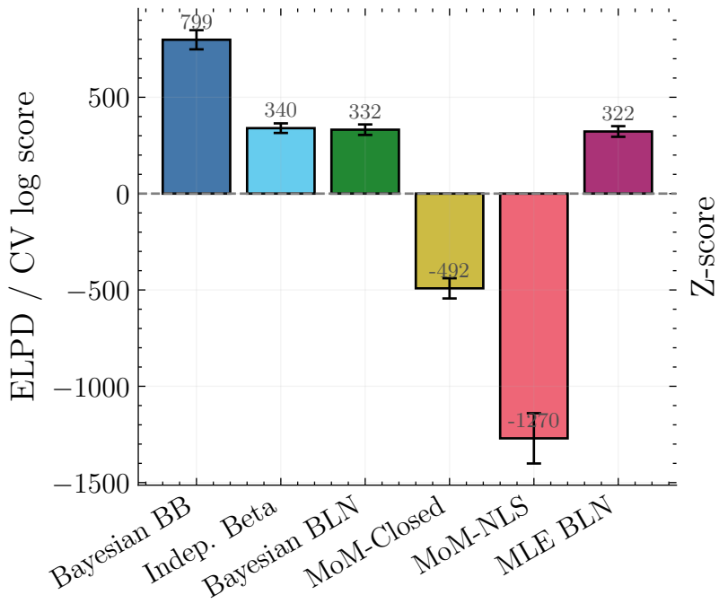
Predictive fit
