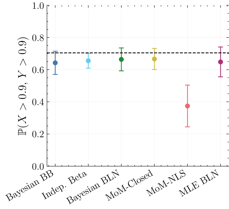
Tail-event calibration
