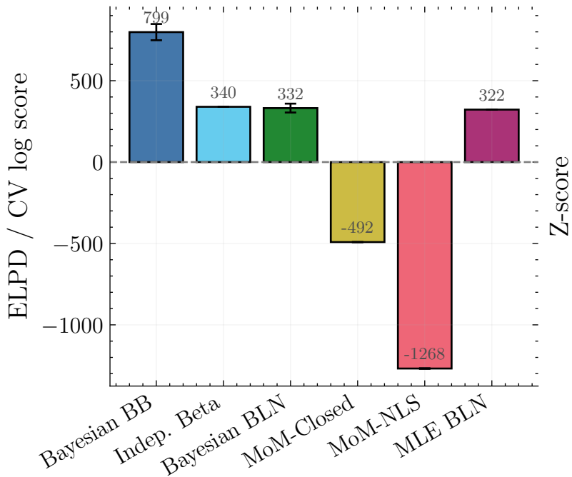
Predictive fit
