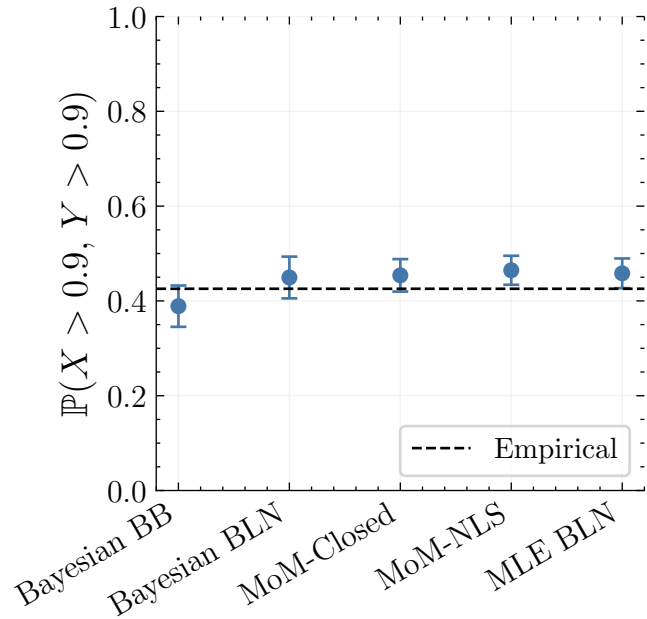
Tail-event calibration
