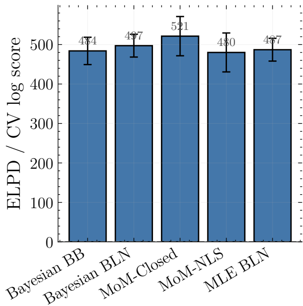
Predictive fit
