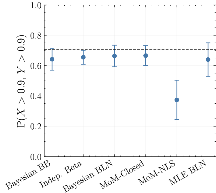
Tail-event calibration
