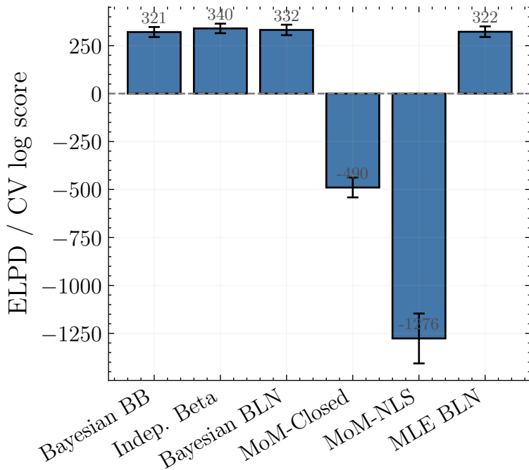
Predictive fit
