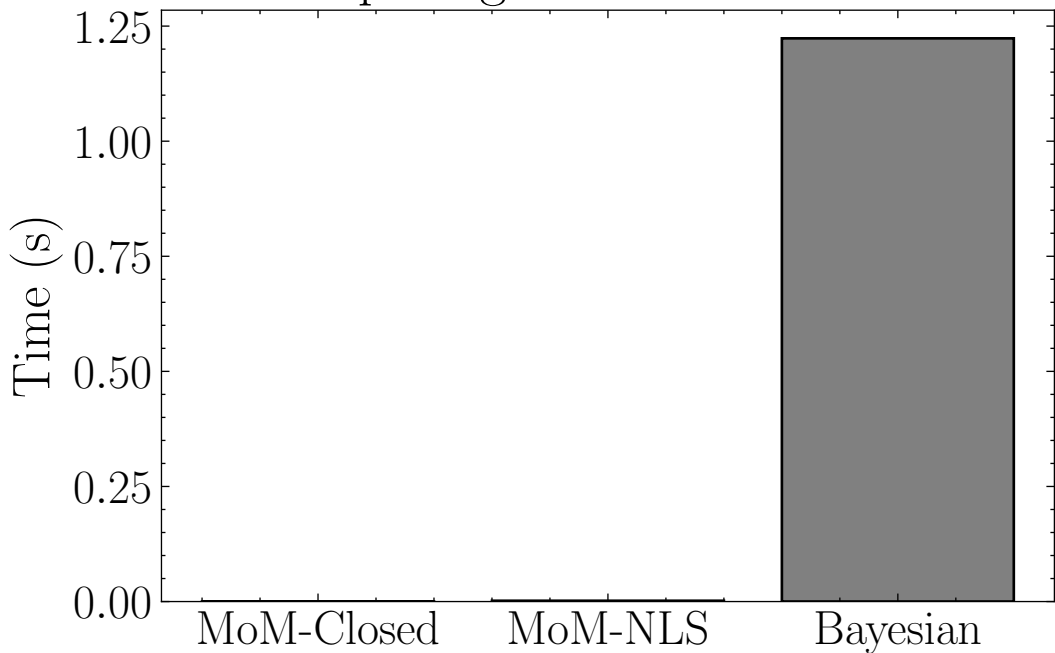
Comparing estimation runtime
