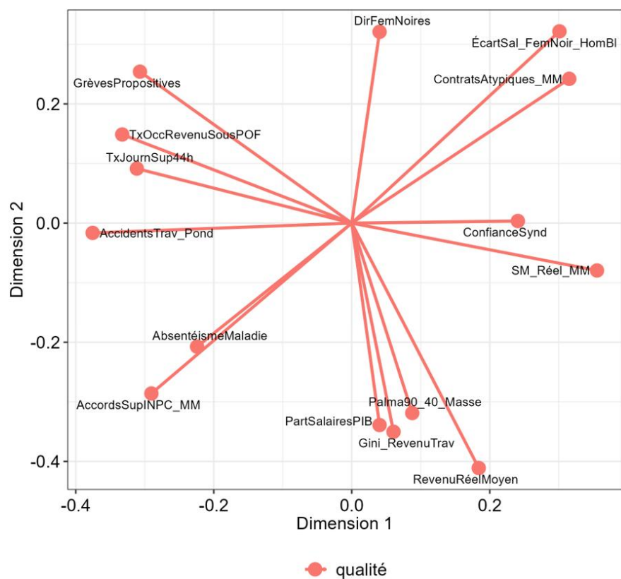
Biplot ACP
