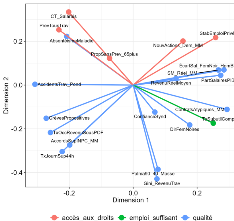
Biplot ACP
