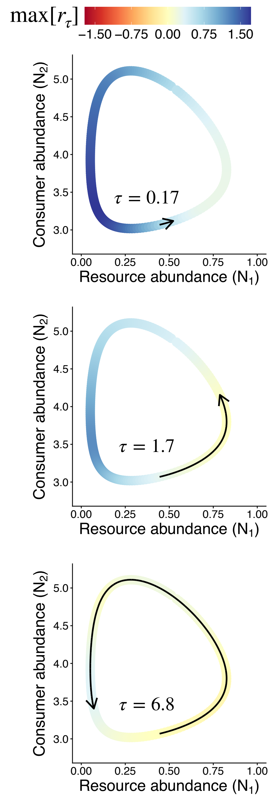
(b) 2-species limit cycle
