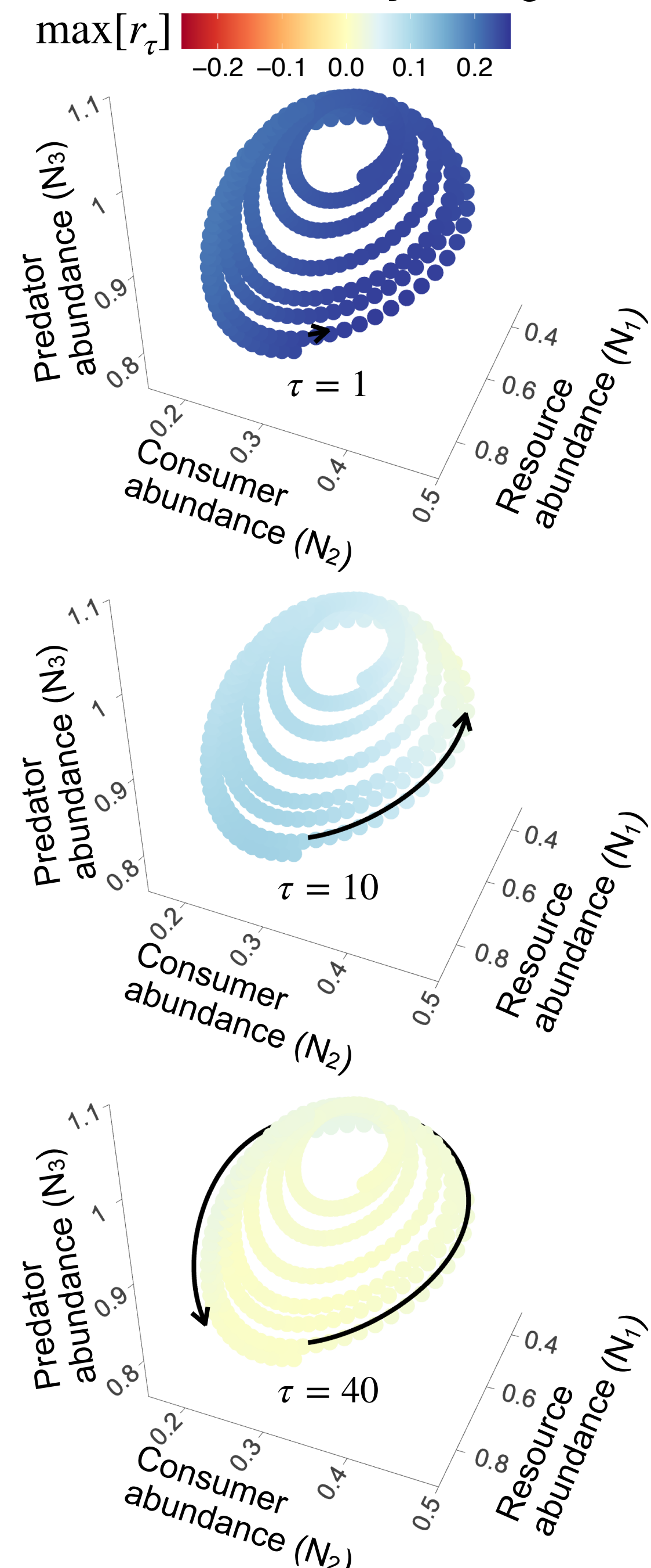
(c) 3-species limit cycle with nonstationary forcing
