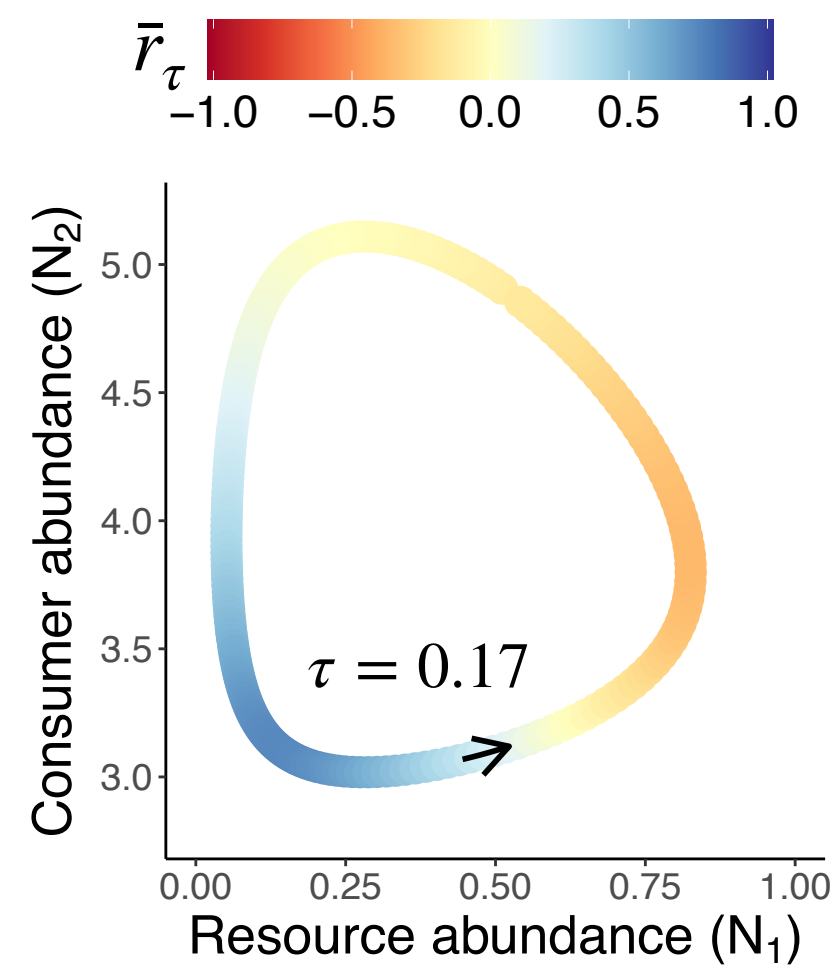
(b) 2-species limit cycle
