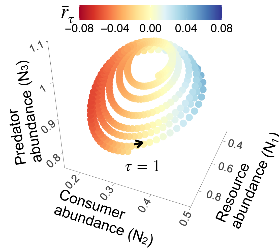
(c) 3-species limit cycle with nonstationary forcing
