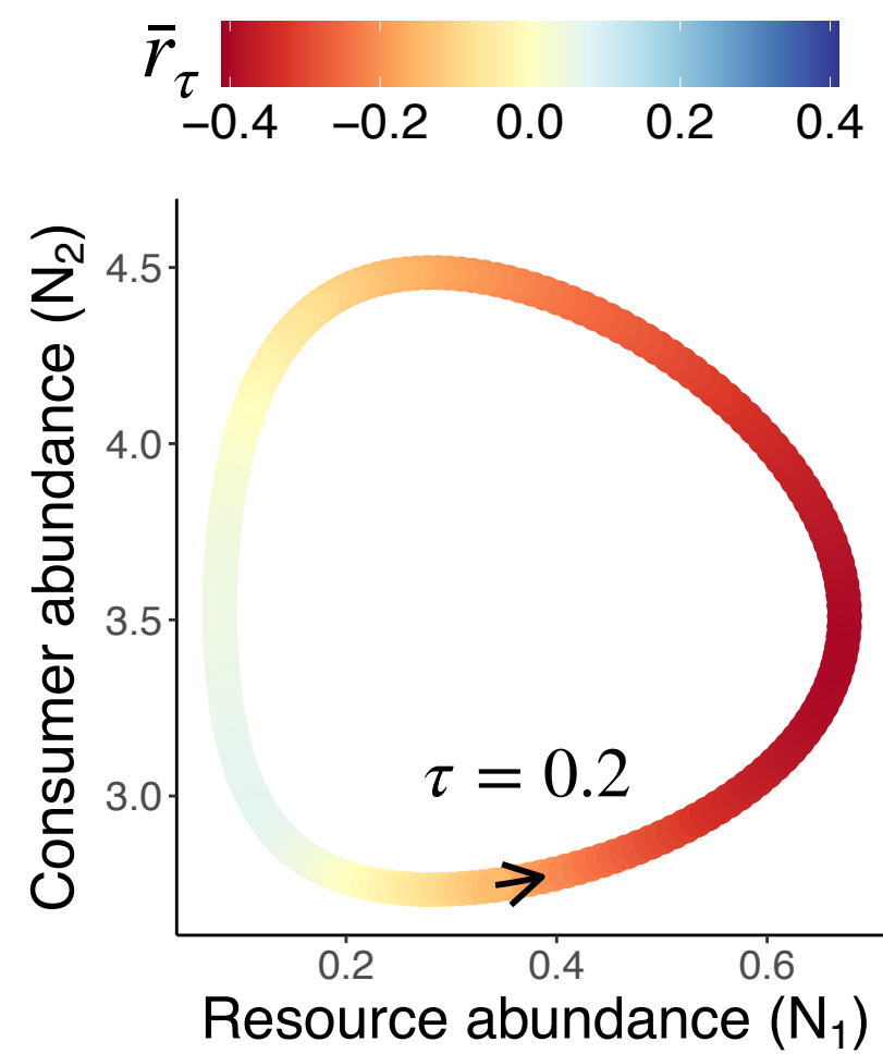
(a) 2-species equilibrium point with periodic forcing
